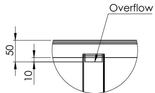
DETAIL B SCALE 1 : 5
